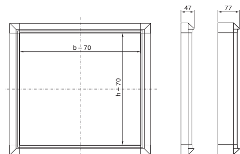
View X for profile height 30
