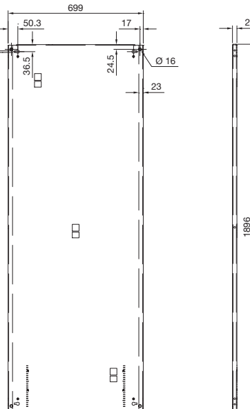
Mounting plate
